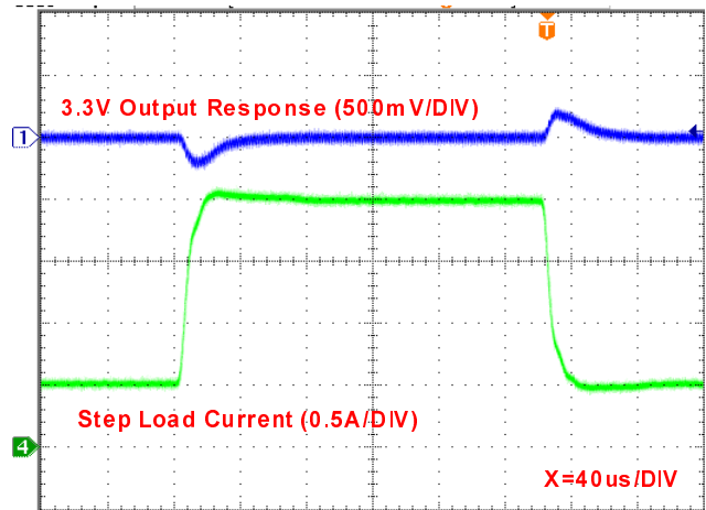
Figure 13(d). 0.5A to 2A step load transient response.
